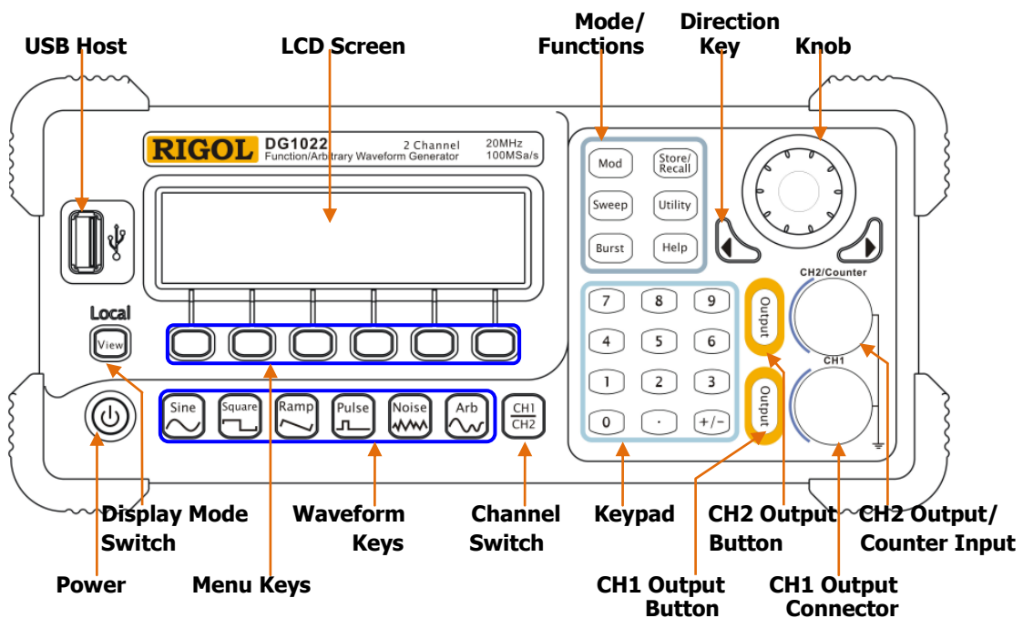
Figure 1-3 Front Panel for DG1022
