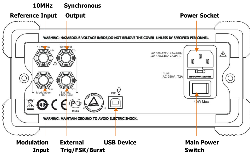
Figure 1-4 Rear Panel for DG1022
